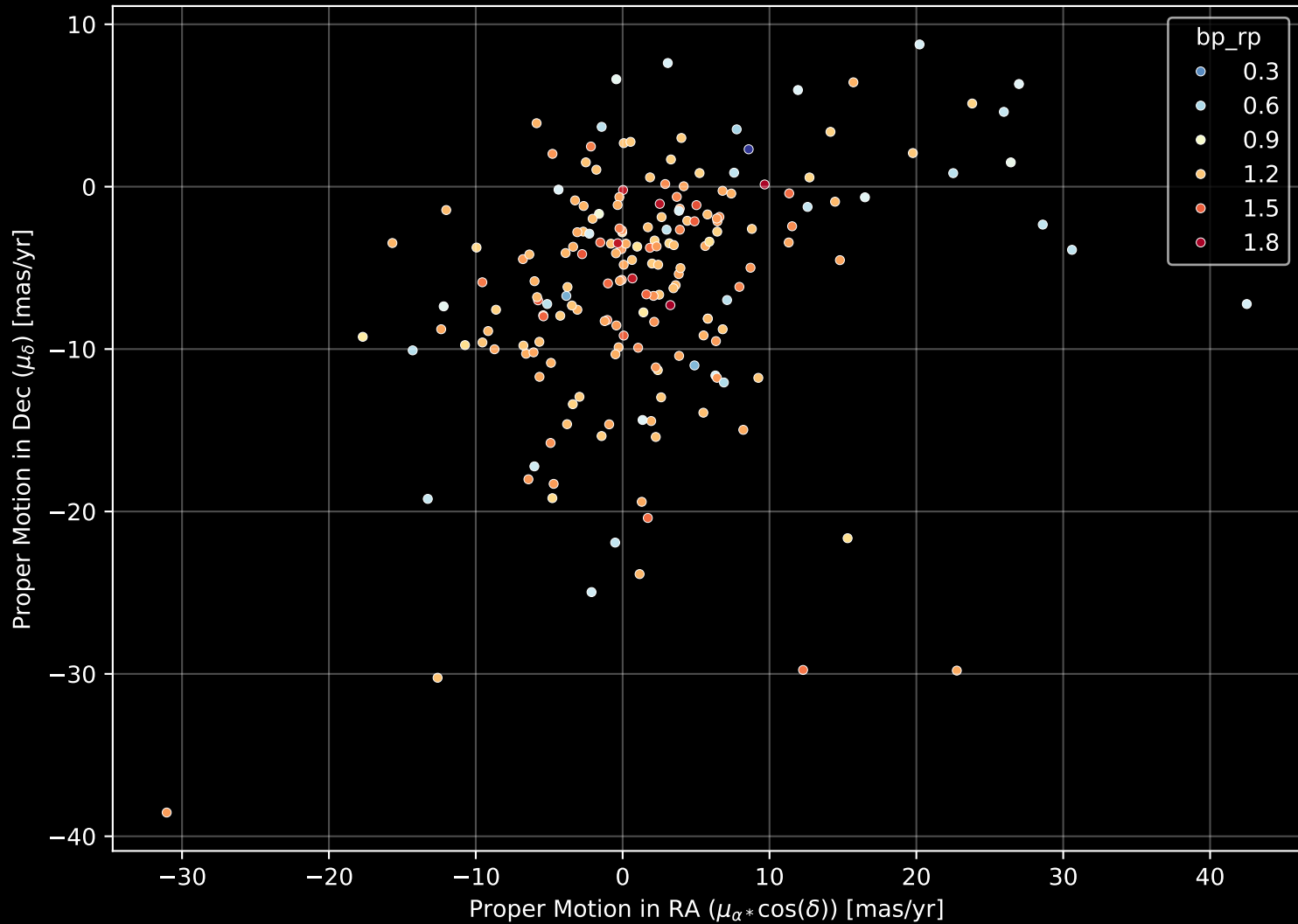
APOGEE DR17 Field: [060-45] Proper Motion Diagram (n= 191)
