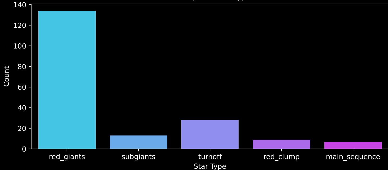
APOGEE DR17 Field: [060-45] Count plot of Star Type
