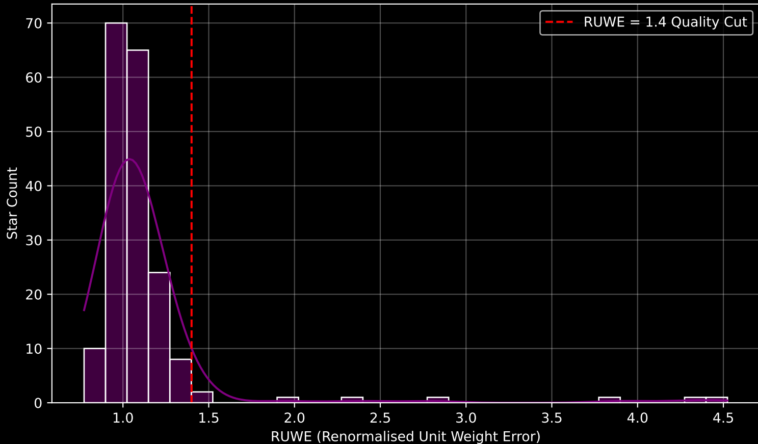
GAPOGEE DR17 Field [060-45] RUWE Distribution (n= 185)
