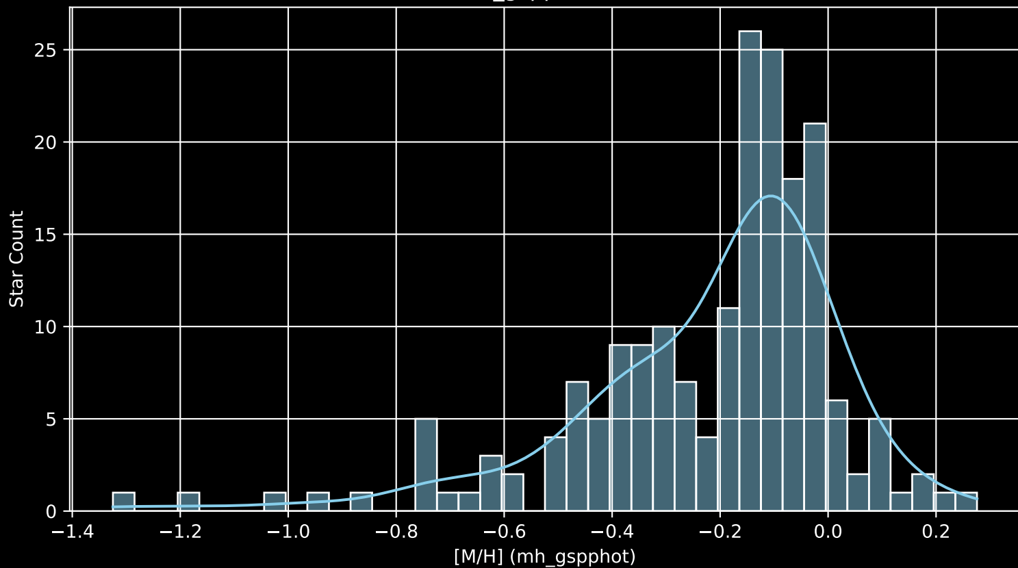
APOGEE DR17 Field: [060-45 [M/H] (mh_gspphot) (n= 191)
