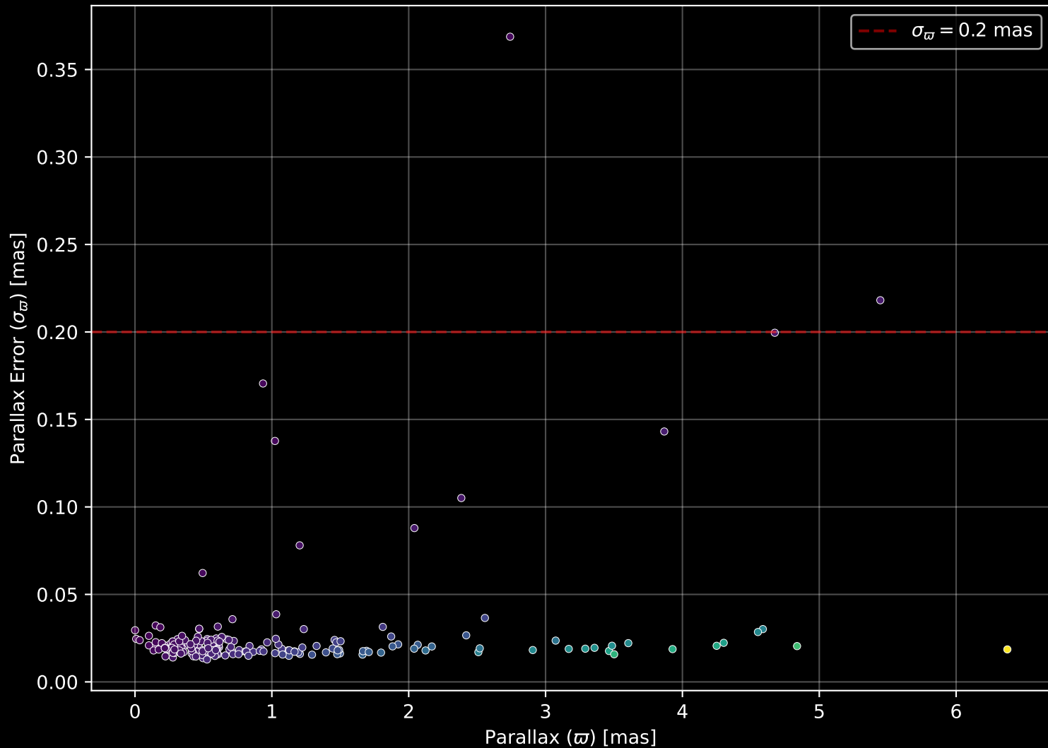
APOGEE DR17 Field: [060-45] Parallax Quality (n= 191)
