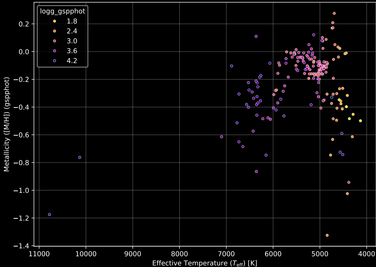
APOGEE DR17 Field: [060-45] Stellar Population Parameters (n= 191)
