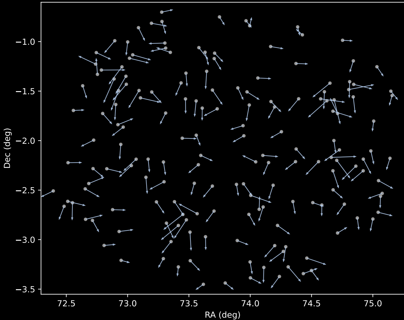
APOGEE DR17 Cluster 1 Proper Motion Vectors (n=169)
